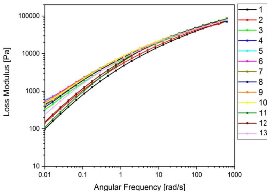
Figure 4. Loss modulus diagram compared to the angular frequency.
