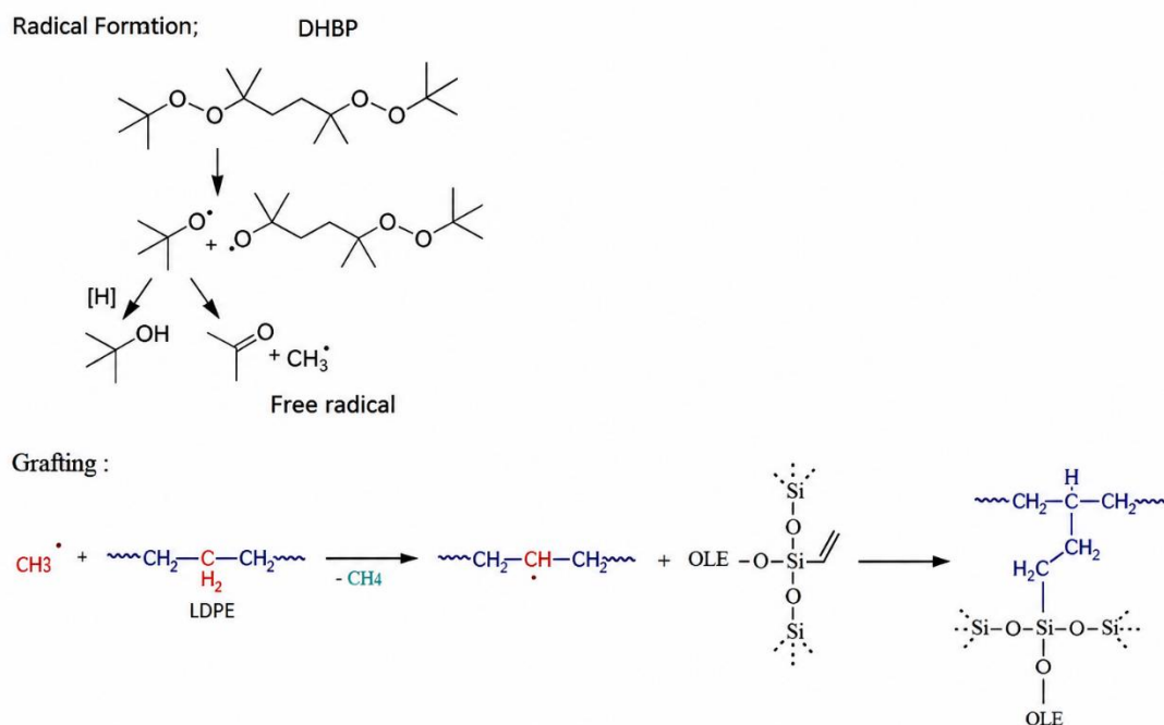
Figure 3. Proposed free-radical grafting mechanism of VTMS-modified oleuropein onto LDPE during peroxide-initiated reactive extrusion.
