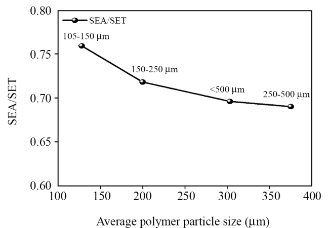
Figure 6. Variation of absorption fraction as a function of initial average polymer particle size in segregated HDPE/CB composites.
