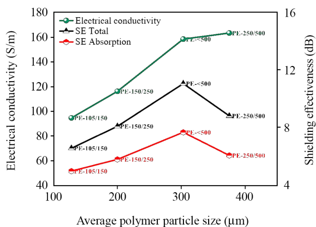
Figure 7. Variation of electrical conductivity and shielding effectiveness with the initial polymer particle size, averaged assuming a linear particle size distribution within the specified range.
