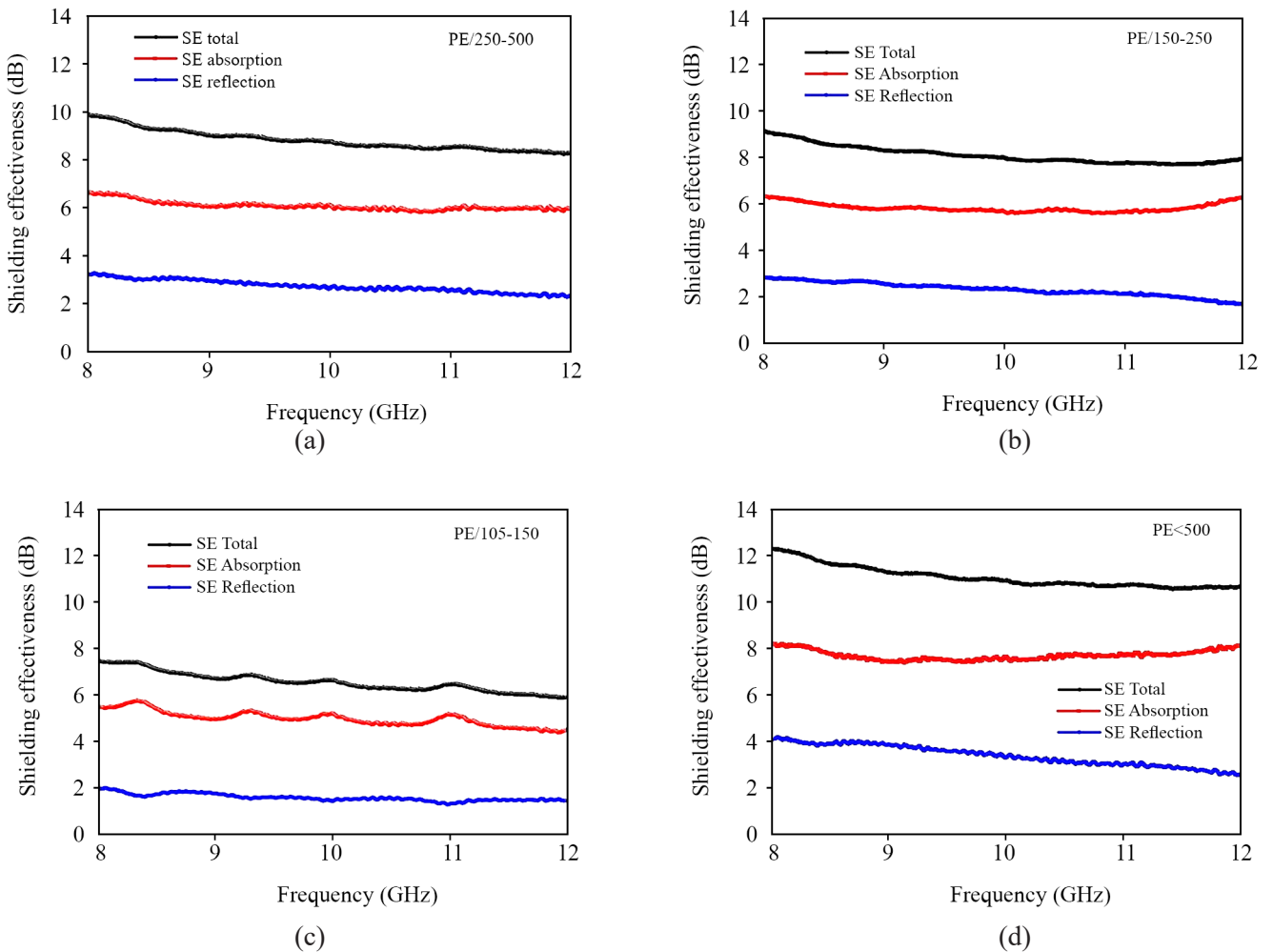
Figure 4. Absorption, reflection and total shielding effectiveness of the segregated HDPE/CB composites in the X-band frequency.
