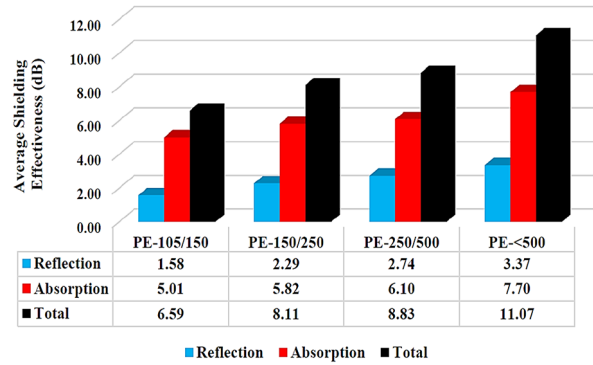
Figure 5. Average total, absorption, and reflection EMI shielding effectiveness of PE/CB segregated composites in the X-band region versus polymer particle size.
