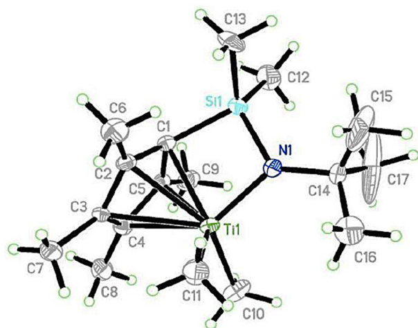
Figure 3. Structure of [\text{t-BuNSiMe}_2(\text{Me}_4\text{Cp})]\text{TiMe}_2 complex.
