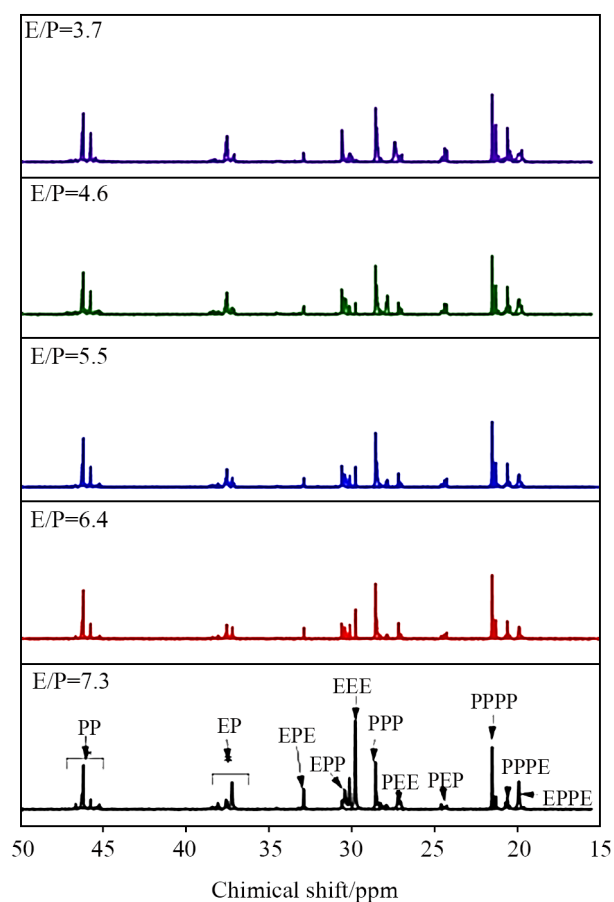
Figure 4. Effect of E/P on sequence distribution of ethylene-propylene random copolymers.
