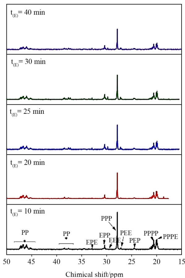
Figure 6. Effect of t_{(E)} on sequence distribution of P-E block copolymers.
