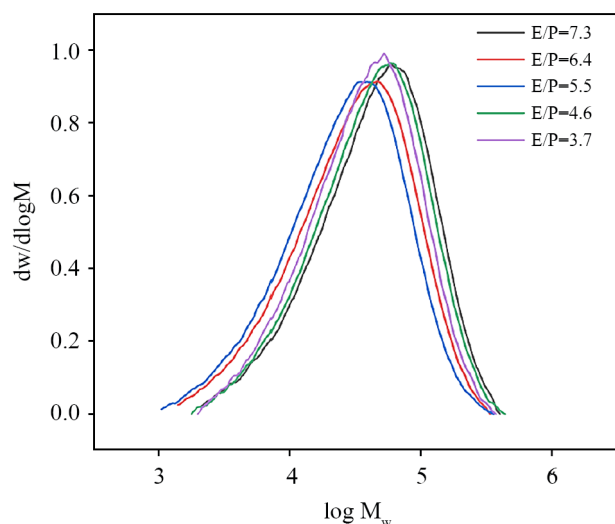
Figure 5. Molecular weight and its distribution curves of ethylene-propylene random copolymers with different E/P.
