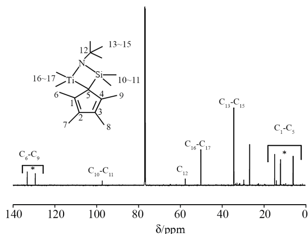
Figure 2. ^{13}\text{C} NMR spectrum of [\text{t-BuNSiMe}_2(\text{Me}_4\text{Cp})]\text{TiMe}_2 .
