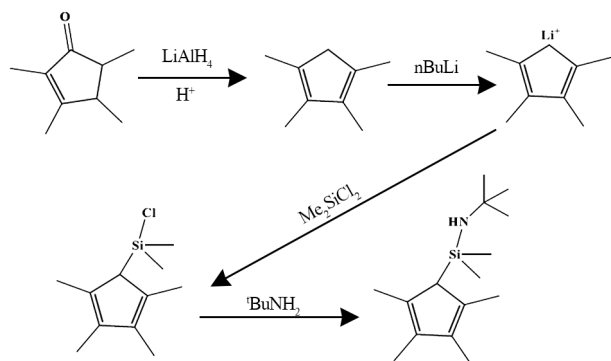
Scheme 1. Synthetic route of \text{Me}_4\text{CpMe}_2\text{Si}(t\text{-BuNH}) .
