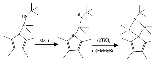
Scheme 2. Synthetic route of [\text{t-BuNSiMe}_2(\text{Me}_4\text{Cp})]\text{TiMe}_2 complex.
