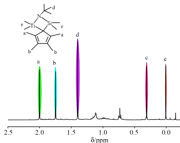
Figure 1. ^1\text{H} NMR spectrum of [\text{t-BuNSiMe}_2(\text{Me}_4\text{Cp})]\text{TiMe}_2 .
