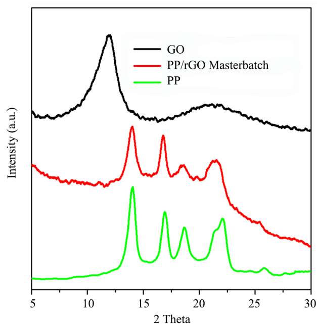
Figure 3. XRD curves of GO, PP/rGO masterbatch and PP.
